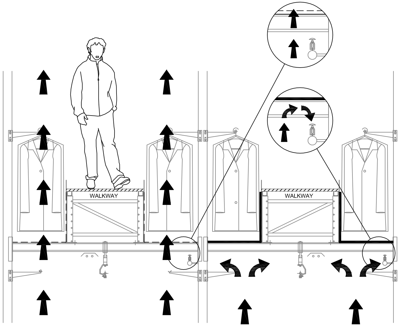
MODIFIED STRUCTURE WITH SUPPLEMENTARY SHEET STEEL SMOKE / HEAT Baffles BELOW WALKWAY LEVEL.
